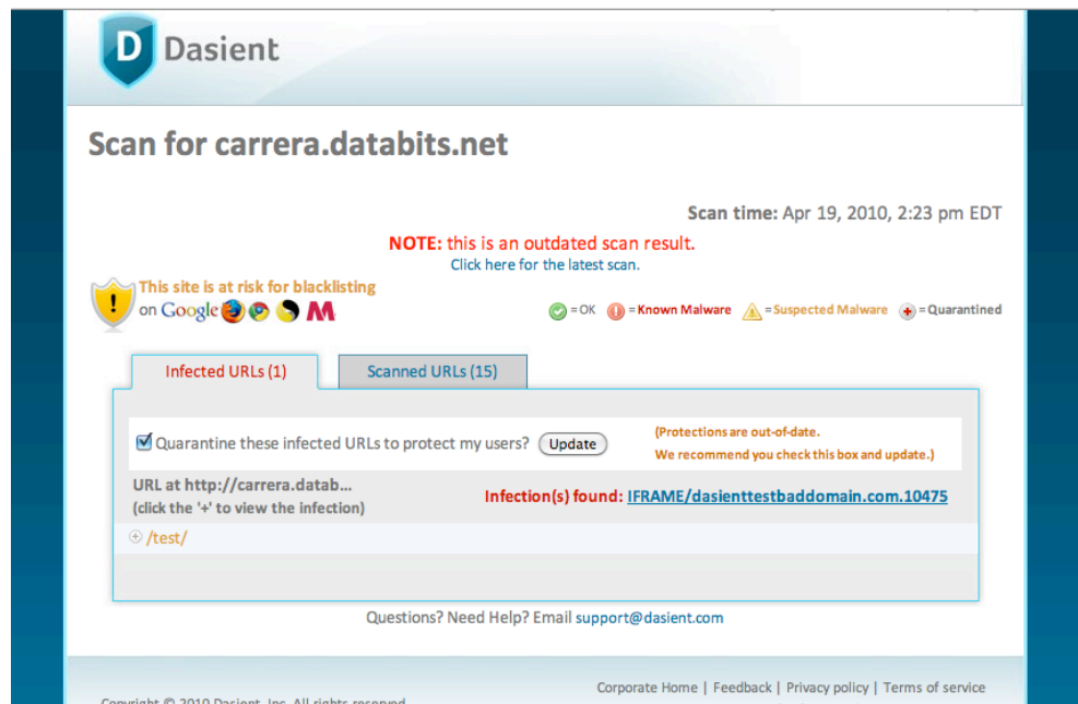
Figure 5. Enabling Quarantining.
